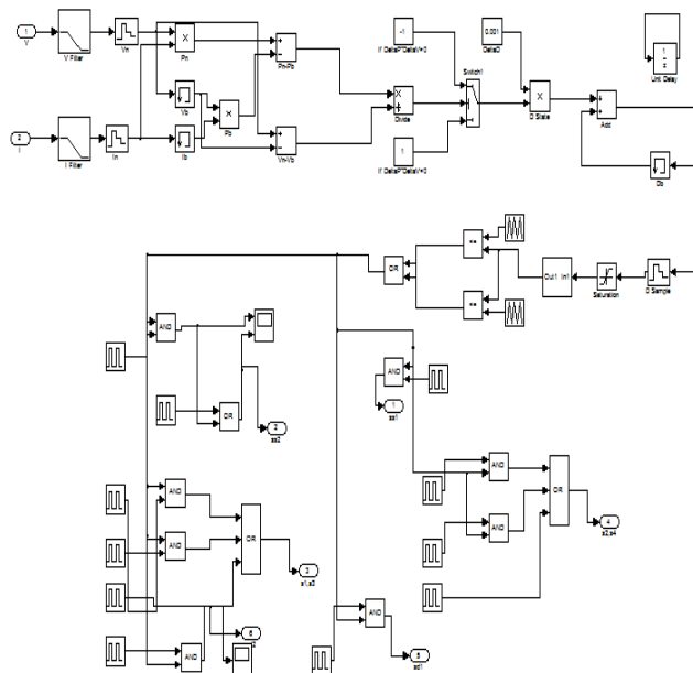
Figure 9. simulink model of MPPT
