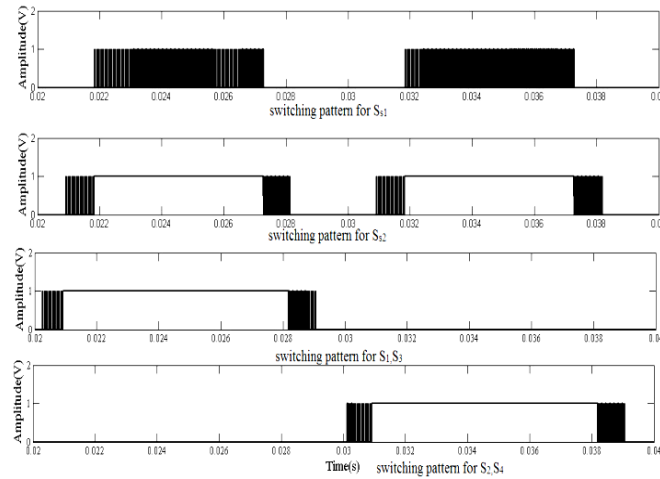
Figure 13. switching pattern for seven level inverter
