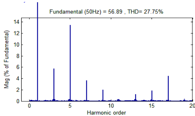
Figure 16.FFT analysis of load voltage of seven level inverter
