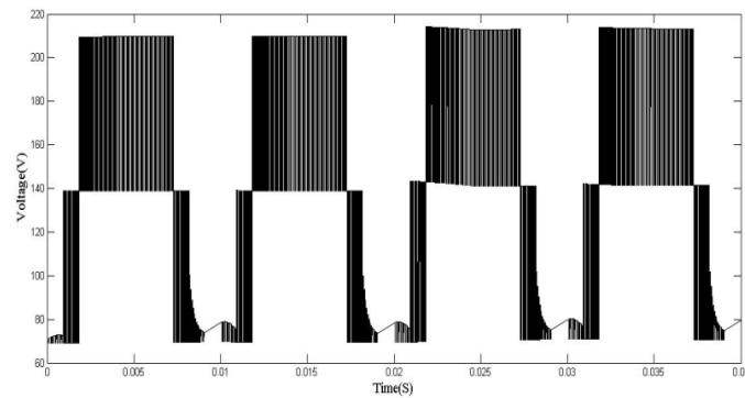
Figure 14. output voltage of capacitor selection circuit
