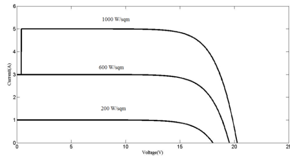
Figure 4. VI characteristics with varying irradiation.
