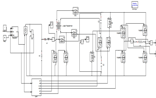
Figure 12. simulink model for PV based MLI with MPPT
