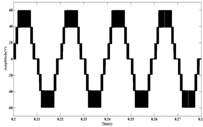
Figure 15.output voltage waveform for PV based MLI with MPPT
