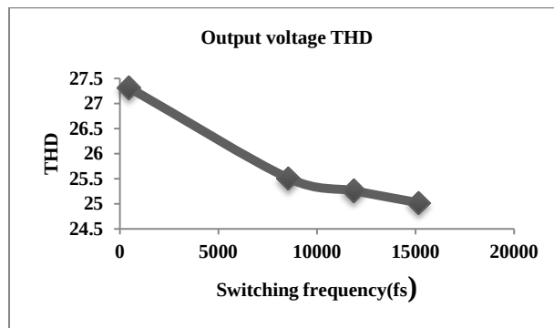
Figure 17. Switching Frequency Vs THD for PV based Dual carrier PWM
