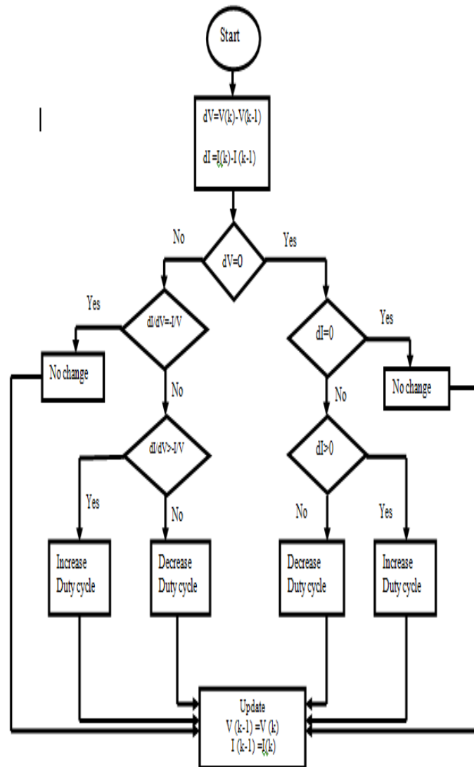
Figure8. flow chart for incremental conductance algorithm
