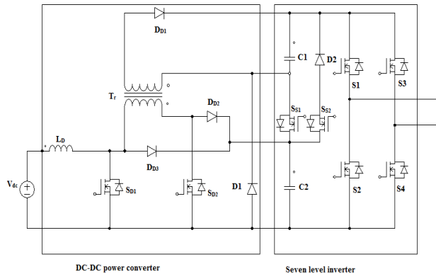
Figure 10 . Seven level inverter together with DC-DC power converter
