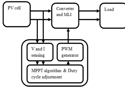
Figure 7. overall block diagram of PV based MLI with MPPT
