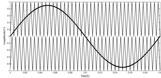
Figure 11. Dual carrier modulation of MLI
