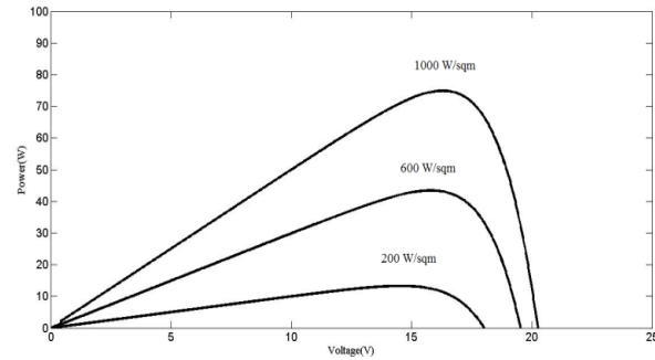
Figure 3. PV characteristics with varying irradiation
