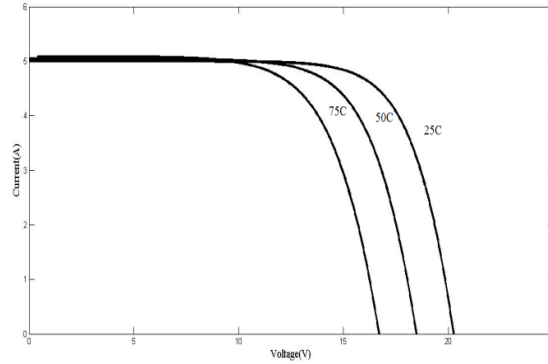
Figure 6. VI characteristics with varying temperature
