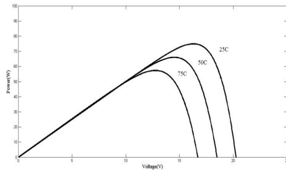
Figure 5. PV characteristics with varying temperature
