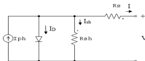
Figure1.PV equivalent circuit
