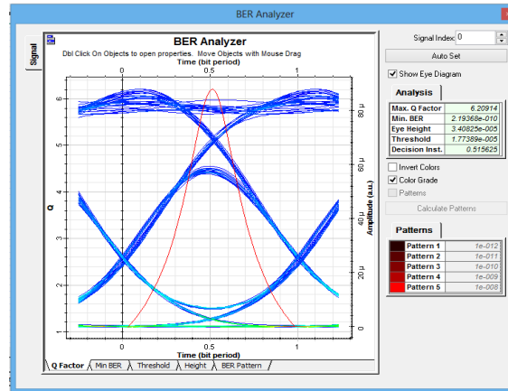
Fig 5: Eye Diagram without Dispersion Compensation
