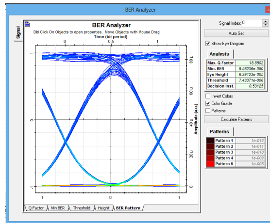
Fig 7: Eye Diagram with Dispersion Compensation
