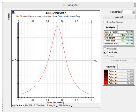
Fig 6: Q-Factor after Dispersion Compensation
