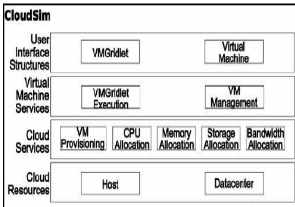
Figure 2 : CloudSim Architecture
