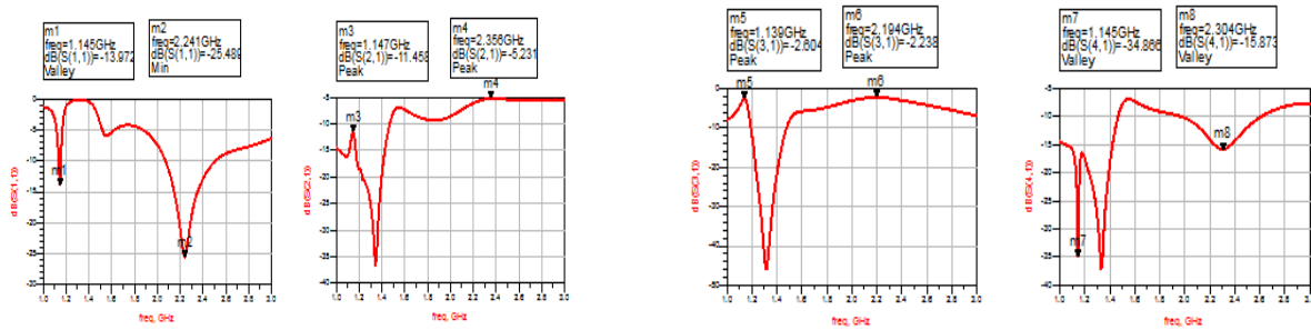
Fig. 7 (a) S_{11} Input Port Fig. 7 (b) S_{21} Throughput Fig. 7 (c) S_{31} Coupled Port Fig. 7 (d) S_{41} Isolation Factor
