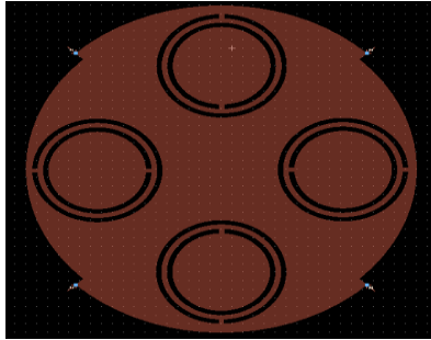
Fig. 6 Configuration of multi-band hybrid coupler with loaded CSRRs
