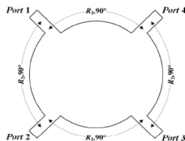
Fig. 1 Configuration of circular sector patch hybrid coupler.
