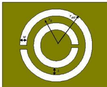
Fig. 2 Configuration of CSRR
